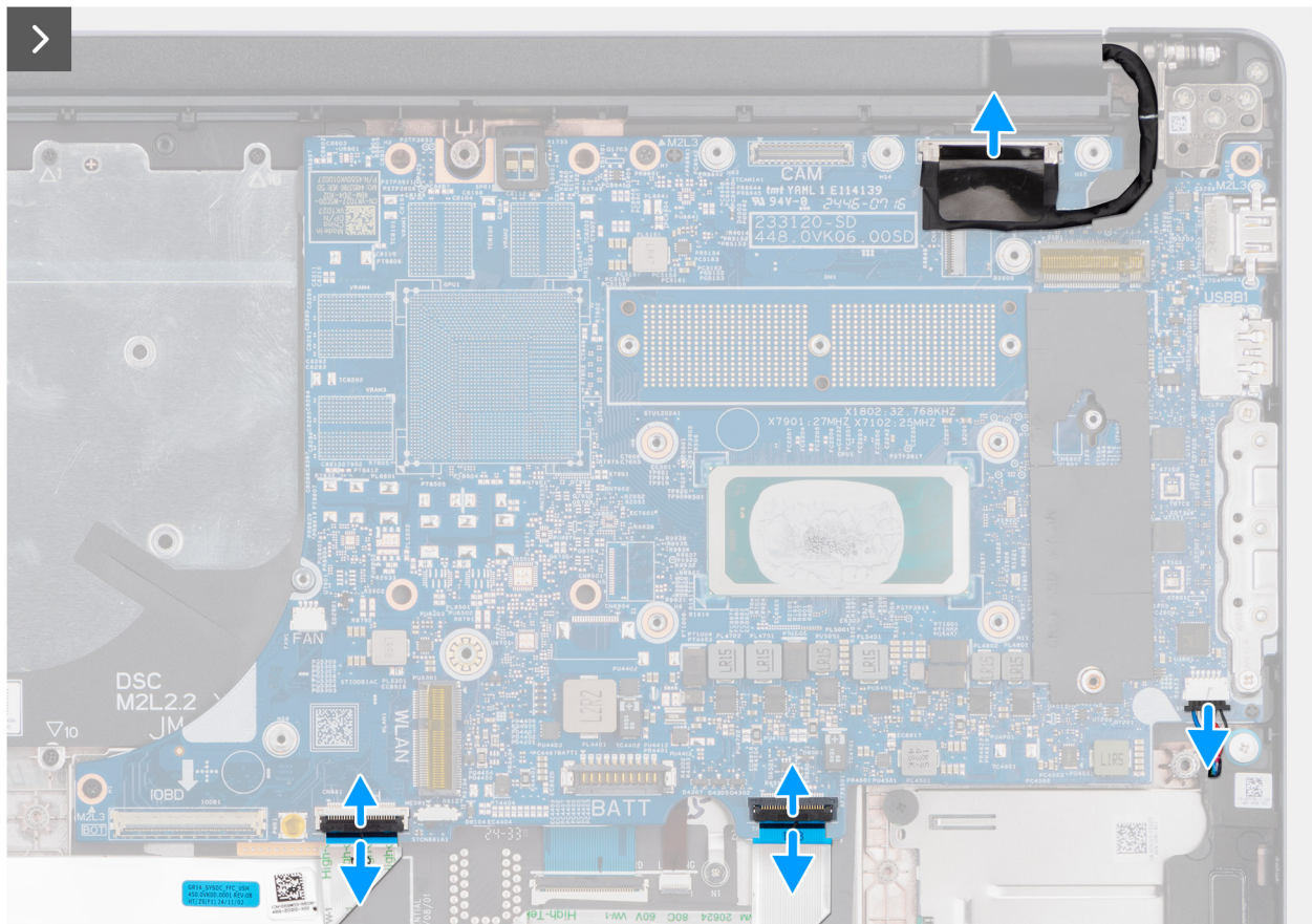
Abbildung 78. Removing the system board
