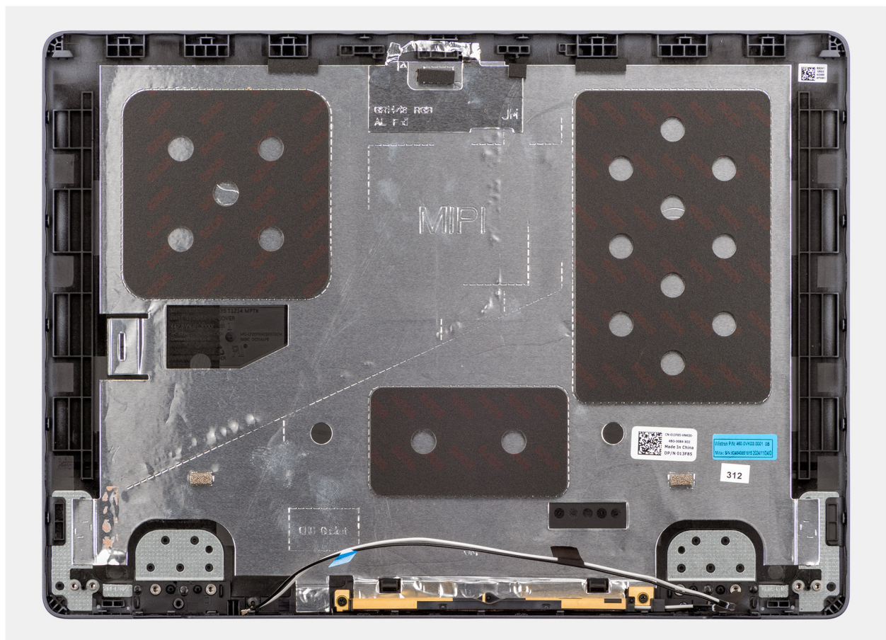
Abbildung 73. Display back-cover and antenna assembly
