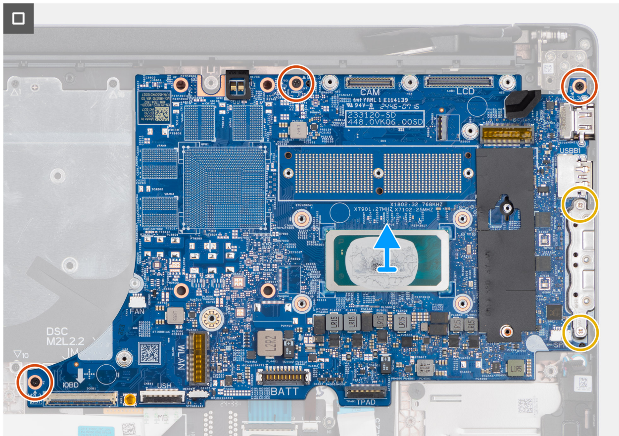
Abbildung 79. Removing the system board
