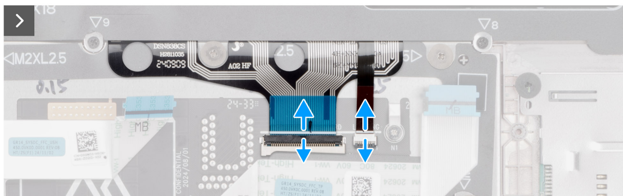
Abbildung 94. Removing the keyboard
