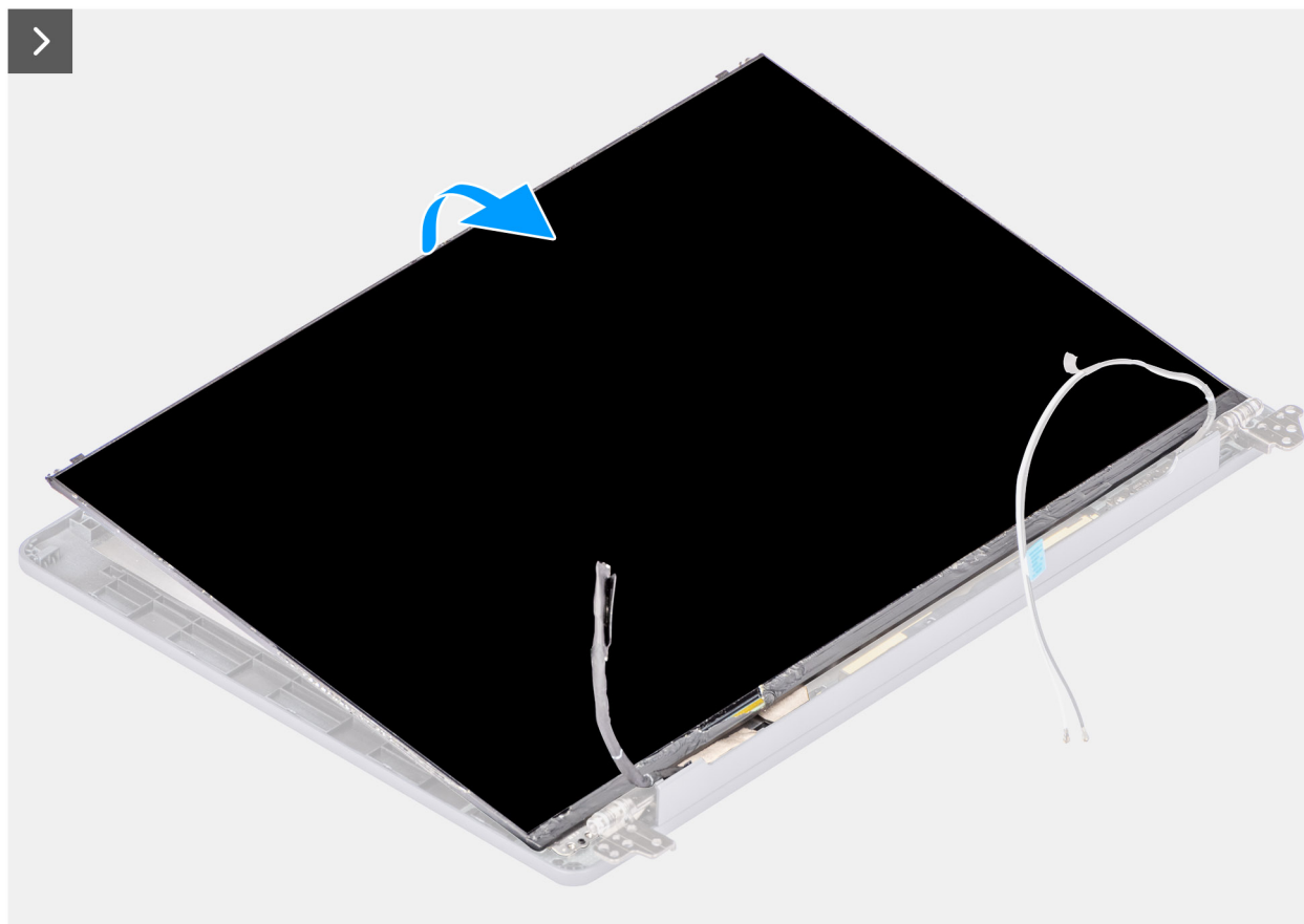
Abbildung 61. Removing the display panel
