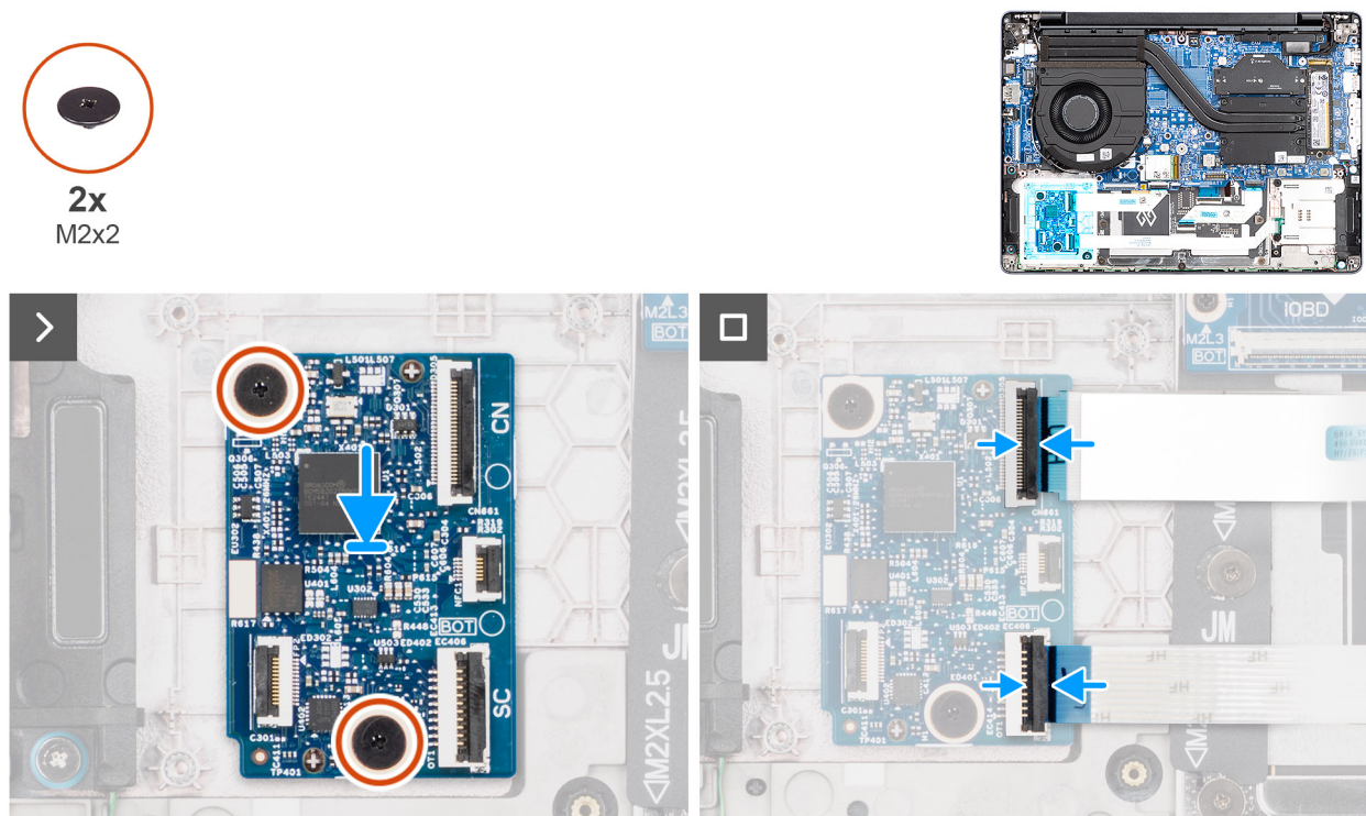
Abbildung 36. Installing the USH board
