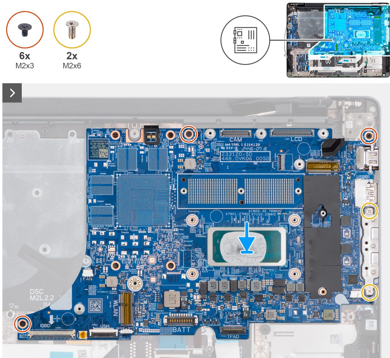
Abbildung 81. Installing the system board
