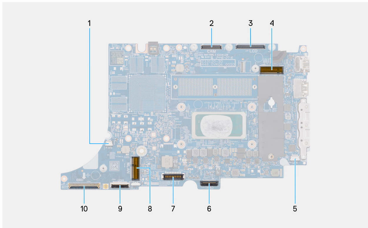
Abbildung 80. System board connectors
