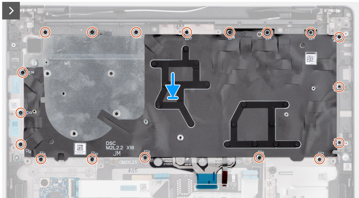
Abbildung 98. Installing the keyboard
