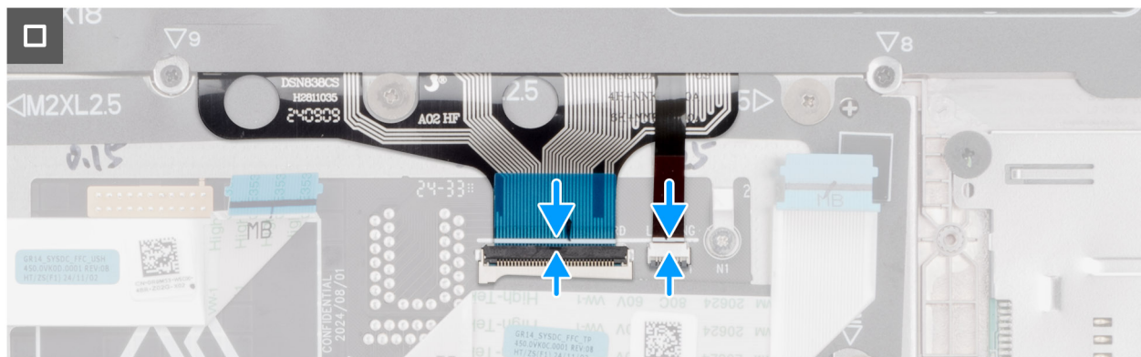
Abbildung 99. Installing the keyboard
